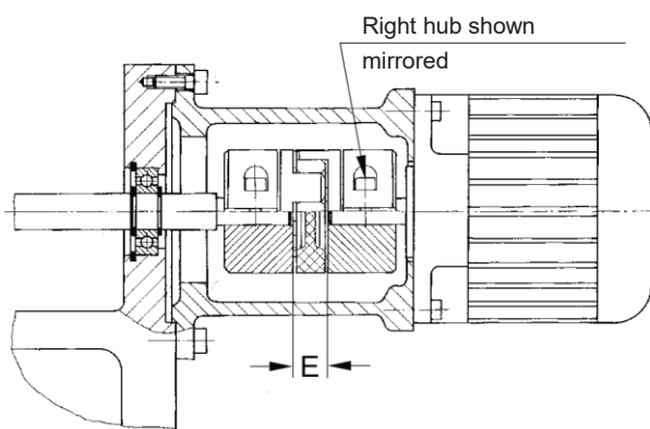
Fig. 15 ROBA®-ES with clamping hubs
