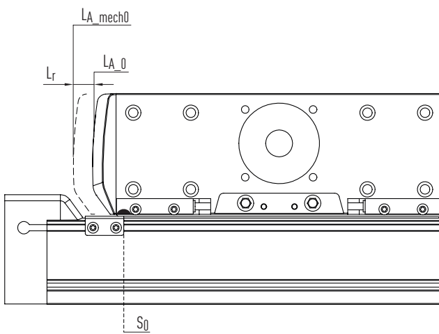
Fig. 24.2 Illustration of reserve stroke (example: cantilever axis HC)
