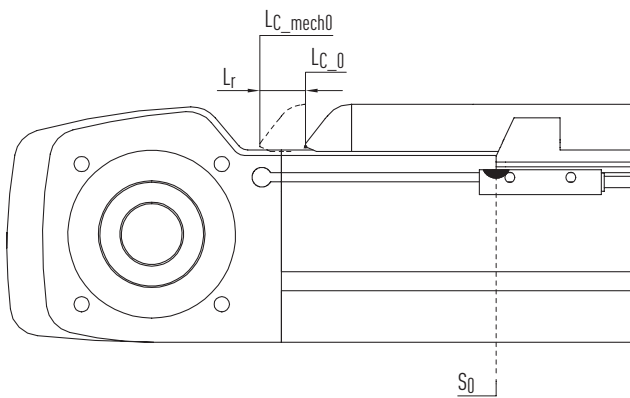
Fig. 24.1 Illustration of reserve stroke (example: linear module HM-B)
