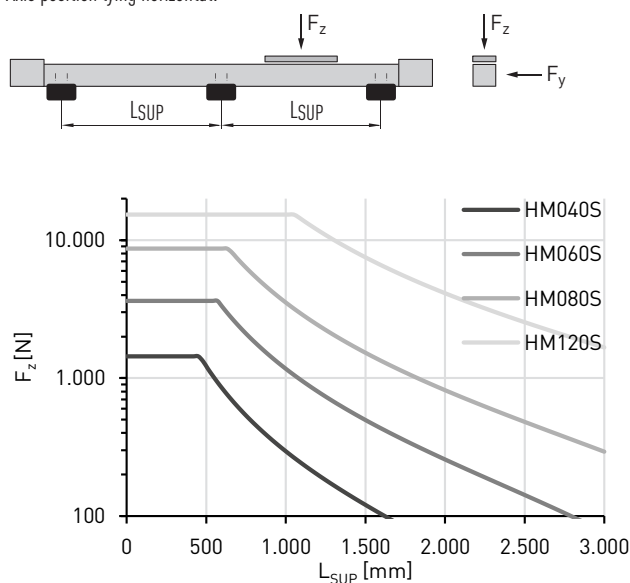
Fig. 3.14 HM-S: Maximum support distance L_{SUP} as a function of force F_z
