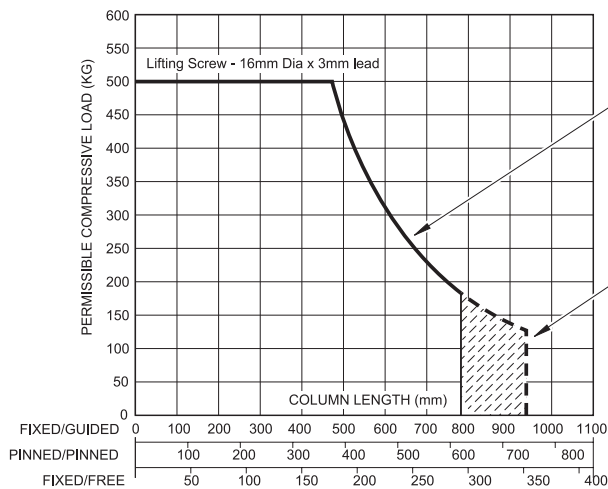
5kN MACHINE SCREW JACK
